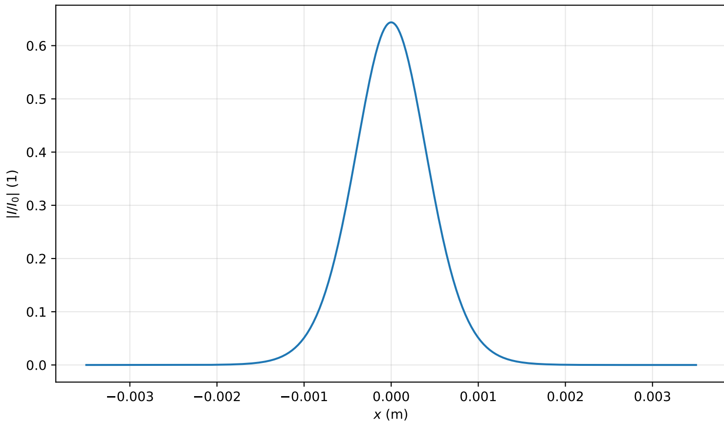
Intensity profile I(x, y = 0, z = 2.309m)/I_0 , P_{in}=0.4P_{cr} , artificial time
